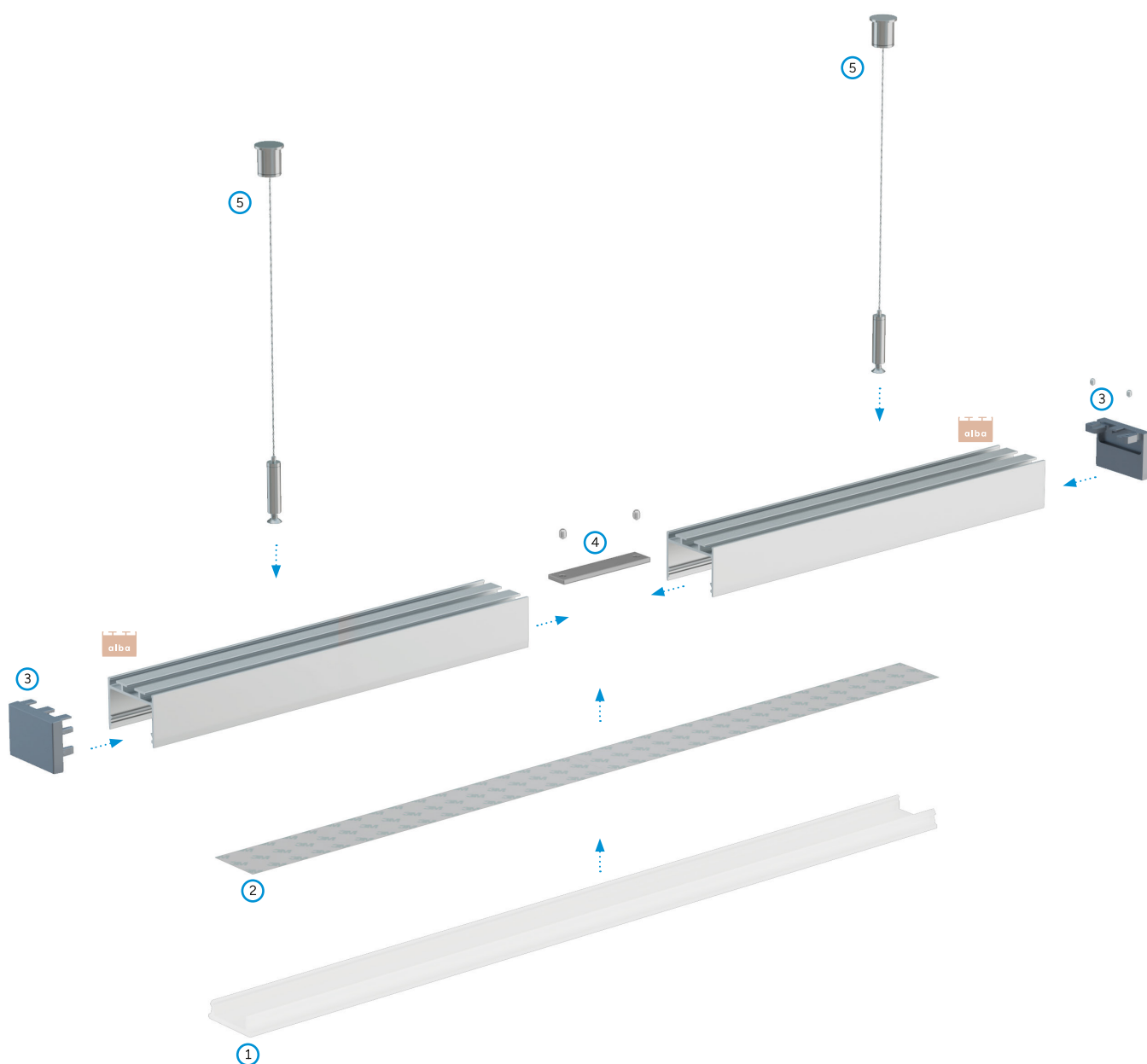
Assembly scheme for elements of the LED lighting system using alba LED profile and (1) midi cover , (2) two LED strips , (3) end caps without holes , (4) straight connector , (5) pendants .
