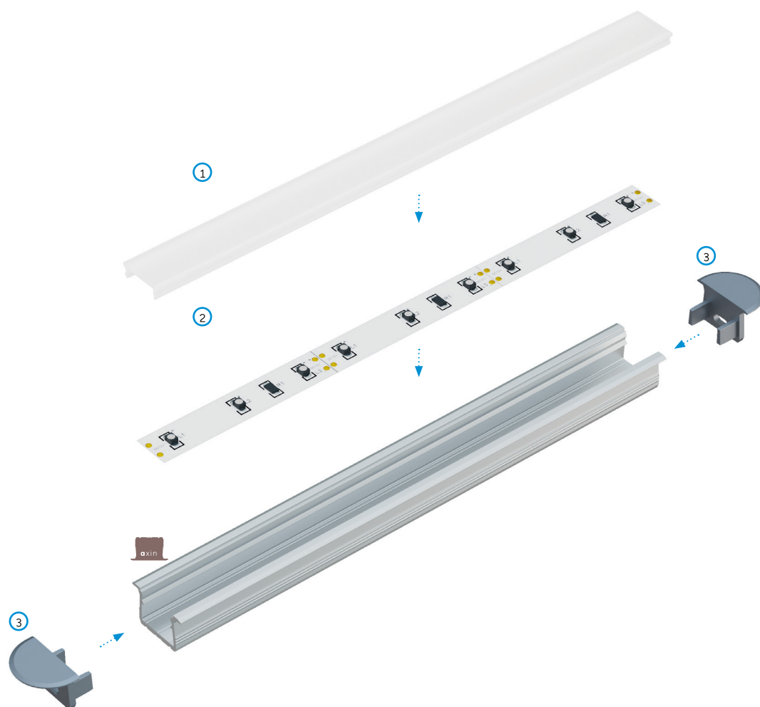
Assembly scheme for elements of the LED lighting system using axin LED profile and (1) nano cover , (2) LED strip , (3) end caps with holes .
