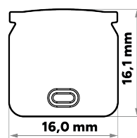
HELSE+ PLASTIC END CAP / ZAŚLEPKA
