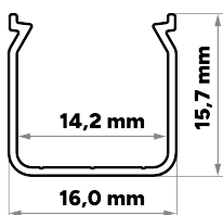
HELSE+ ALUMINIUM LED PROFILE / PROFIL LED
