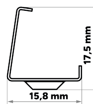
BARDE+ METAL MOUNTING CLIP / UCHWYT
