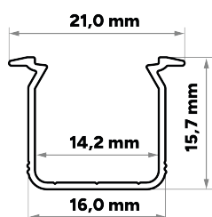
SKAGEN+ ALUMINIUM LED PROFILE / PROFIL LED
