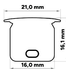
SKAGEN+ PLASTIC END CAP / ZAŚLEPKA
